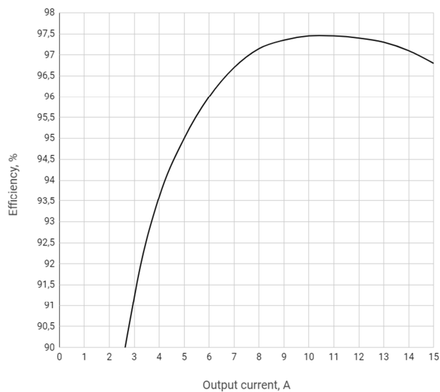
Figure 2 – Efficiency vs. output current at full load
