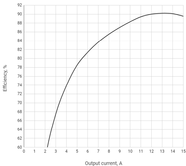
Figure 4 – Efficiency vs. output current at light load
