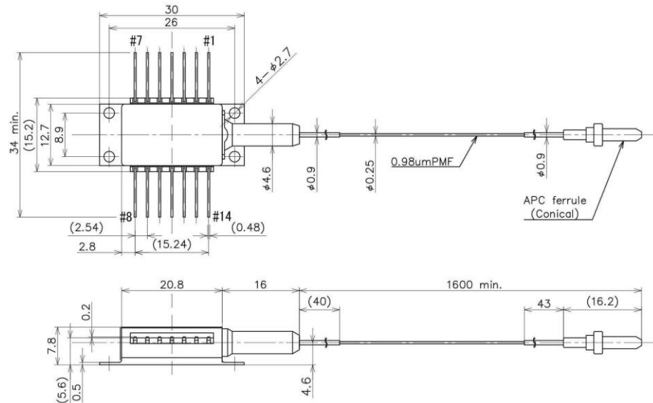
(b) 250um fiber diameter and ferrule type (QLD106L-6430-11)
