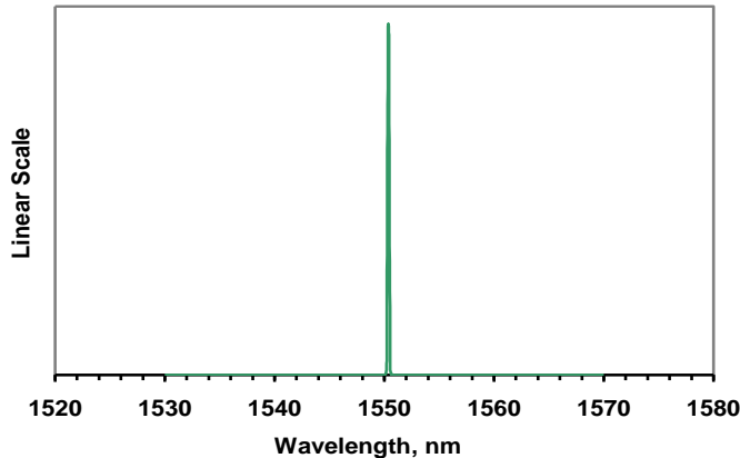
Emission Spectrum
