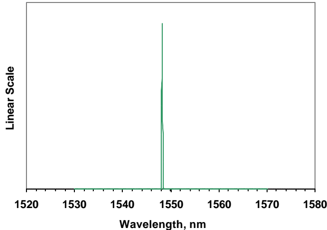
Emission Spectrum
