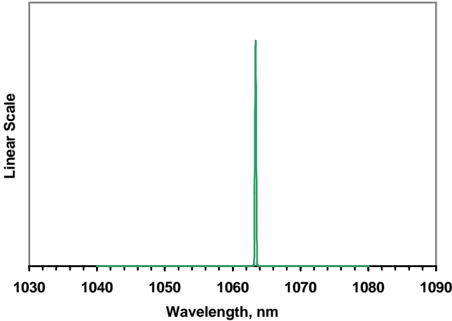
Emission Spectrum
